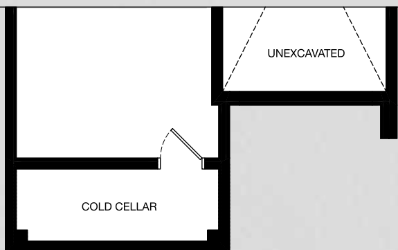
Basement Floor Elev. 'A'
