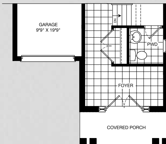
Partial Main Floor Elev. 'B'
