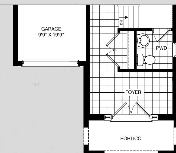
Partial Main Floor Elev. 'C'
