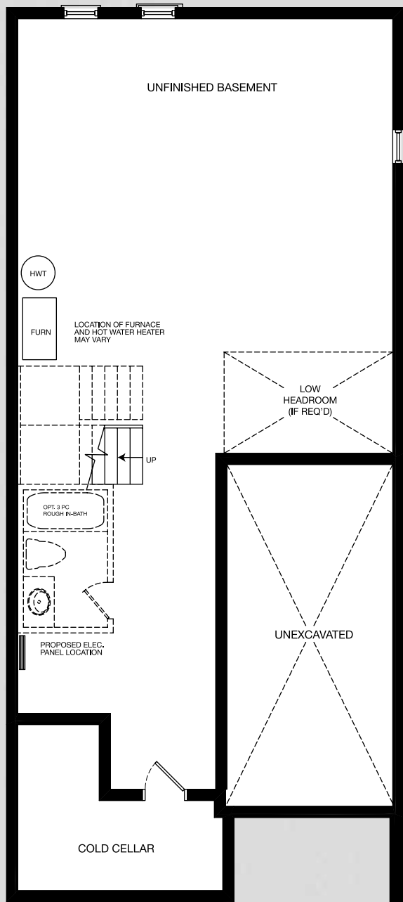
Basement Floor Elev. 'A'
